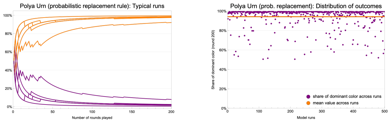
Figure 3: Outcome for a modified Polya urn where the probability for the new ball to have color x is proportional to the current share of balls that are of color x .
